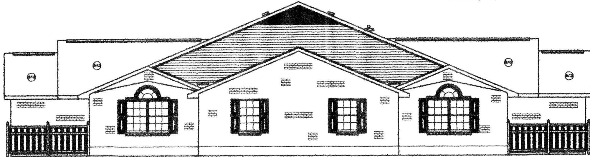
SIDE ELEVATION FOR UNITS W/ SLAB
