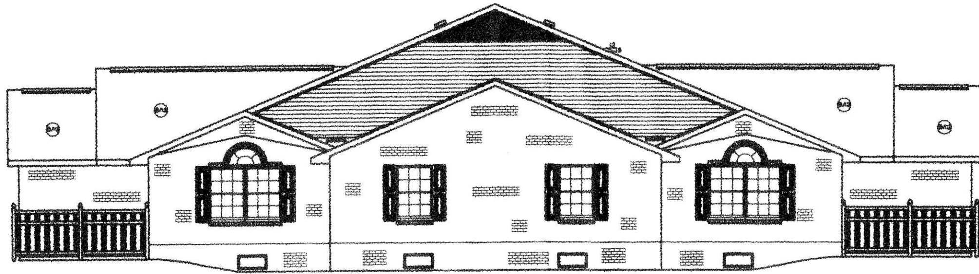
SIDE ELEVATION FOR UNITS W/ BASEMENT
